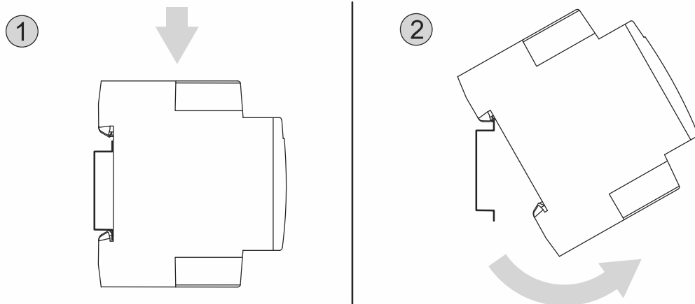
Fig. 8: Removal from the mounting rails
